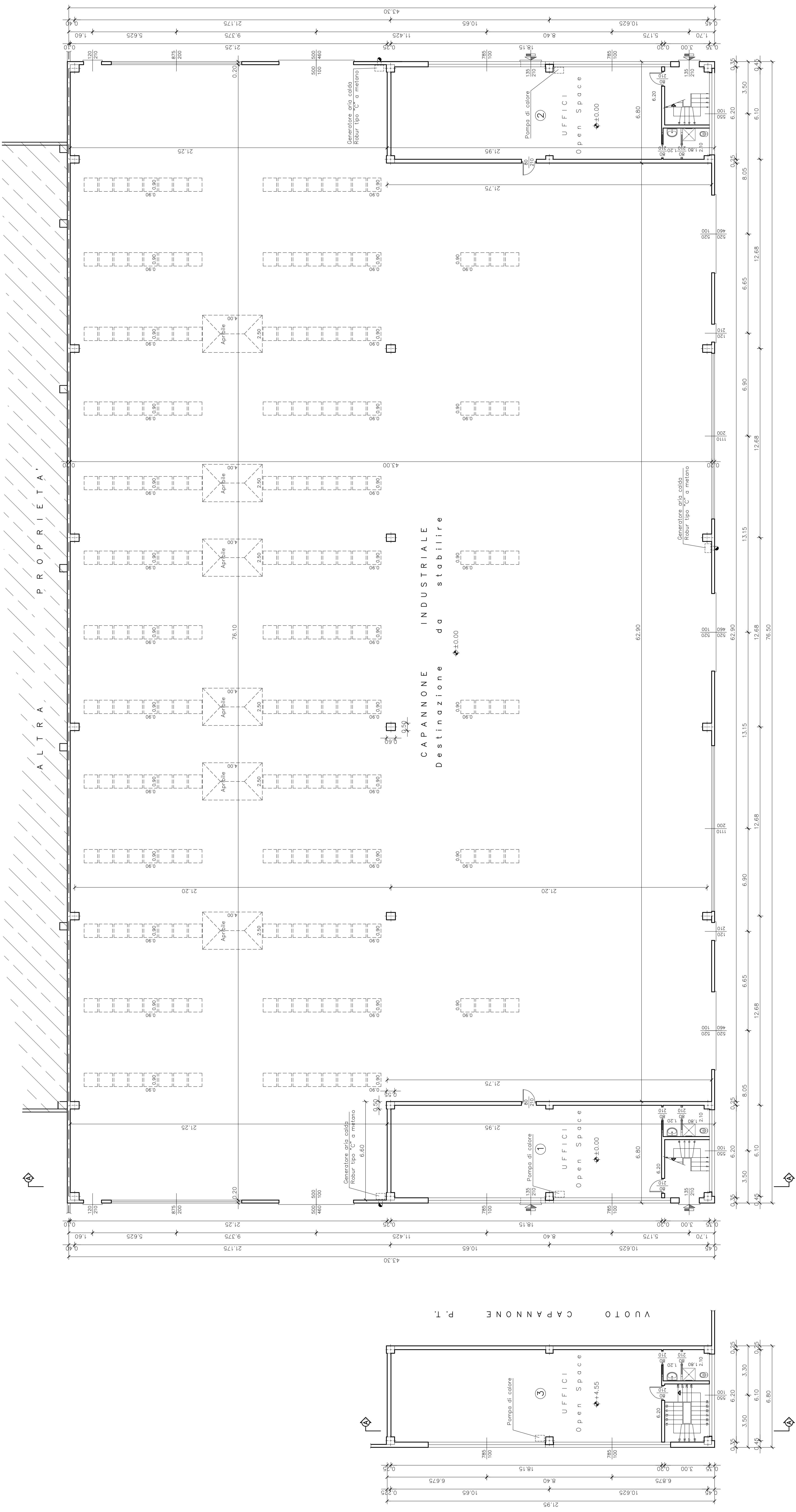
PIANTA PIANO 1*
